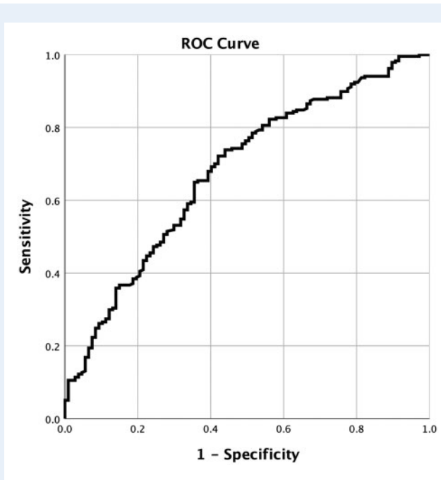
Figure 2. Receiver operating characteristic curve of the prediction model. Area under the curve = 67.6% (95% CI = 64.9–70.3%), indicating reasonable discriminative performance.
