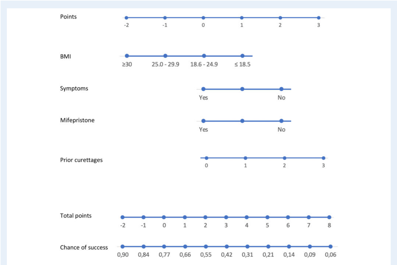
Figure 5. A nomogram for prediction of the chance of successful medical treatment in case of early pregnancy loss. Each factor (BMI, symptoms, mifepristone, prior curettages) has a score on the point scale, which can be determined by drawing a vertical line from the factor scale to the point scale. The estimated chance of success is calculated by adding all points to generate a point total, locating this score on the total point scale and subsequently the corresponding chance of success.
